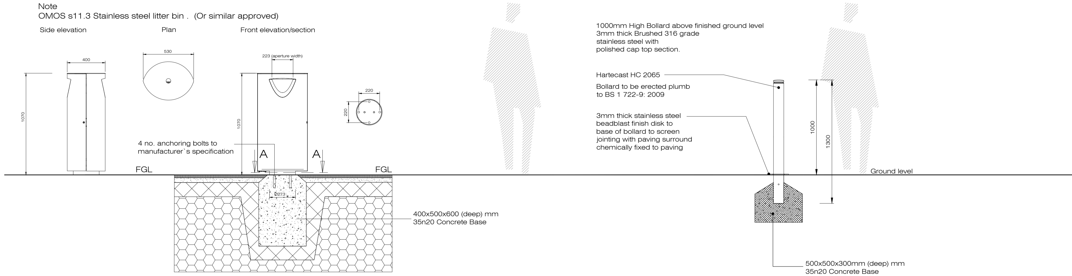
Detail D 01 Drawing LD-04-PP Litter bins to open space area Scale @ 1:20
